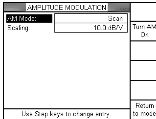
Figure 2-23: Scan Modulation Selection
