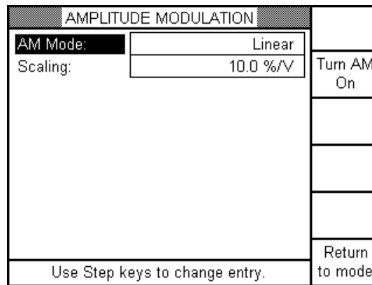
Figure 2-21: Amplitude Modulation Selection
