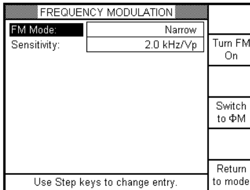
Figure 2-25: Frequency Modulation Selection
